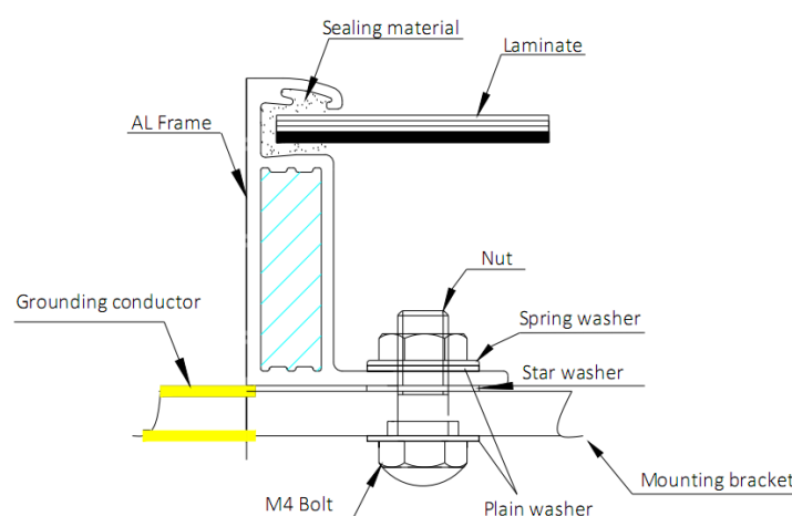
Fig. 10-1 Grounding
